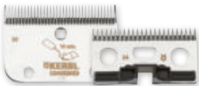
18914 Schermesser-Set R2 Standard-Feinschur
